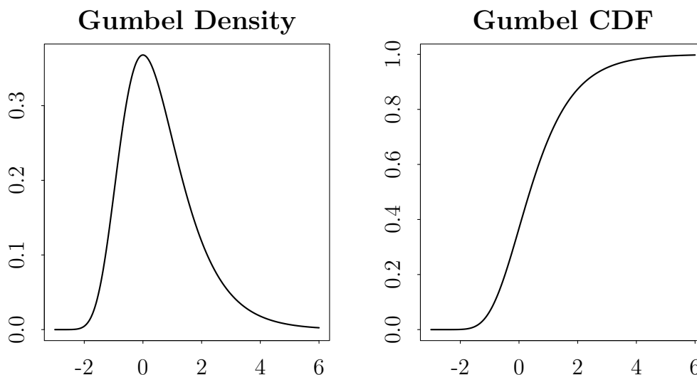
Figure 4.1: The density and CDF of Gumbel, aka Type I Extreme Value, random variable. Left panel: f(z) = \exp(-z) \exp\{-\exp(-z)\} . Right panel: F(z) = \exp\{-\exp(-z)\} .
